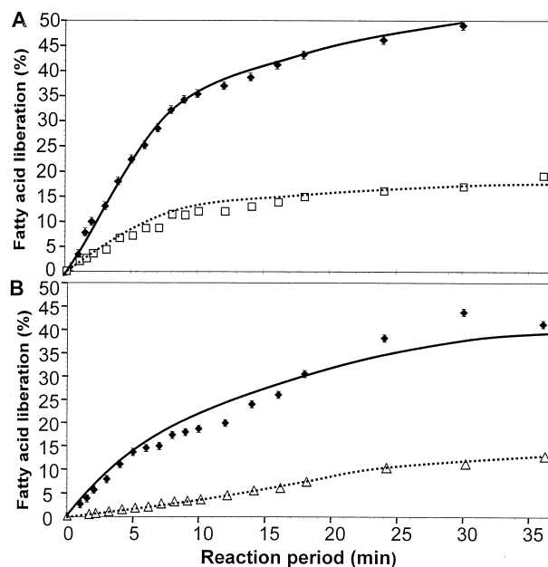
Fig. 2. sn -2 cleavage of equimolar mixtures of non-lipoxygenated (P APC ) and 15-lipoxygenated (P APC -OOH and P APC -OH) substrates (12.5 µM each) by the sPLA 2 from bovine pancreas. A: Equimolar mixture of P APC and P APC -OOH. B: Equimolar mixture of P APC and P APC -OH. The values for the liberation of AA (◆), 15-HpETE (□) and 15-HETE (△) are expressed as molar percentages of the initial total amount of phospholipids in the sample. AA values represent the mean ± S.D. of four separate experiments. The values of 15-HpETE and 15-HETE represent the mean of two experiments. Other conditions as in Fig. 1.
