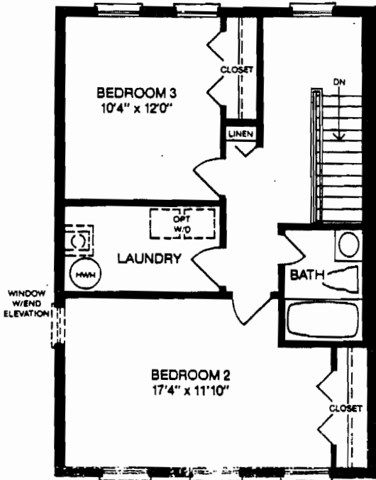
THIRD FLOOR PLAN W/ELEV. 5, 6
