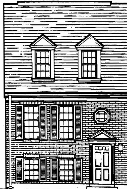
FRONT ELEVATION 8
