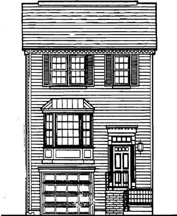
GARAGE FRONT ELEVATION 9
