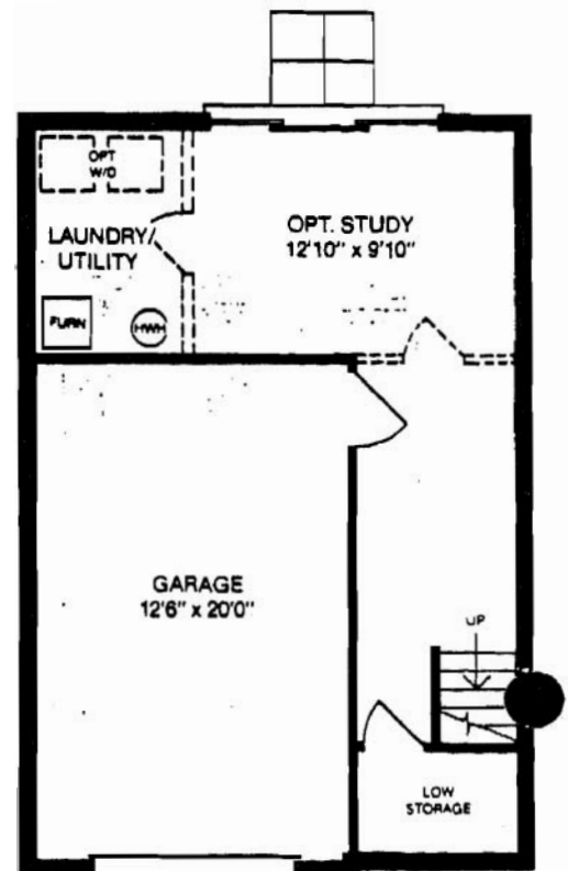
GARAGE LOWER LEVEL FLOOR P U N
