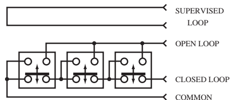
Circuit # - C1
