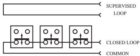
Circuit # - C1
