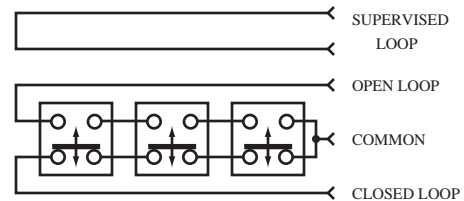
Circuit # - C2
