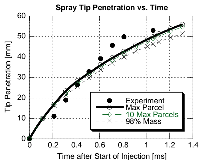
Figure 3. Comparison of Spray Tip Penetration Measurements
